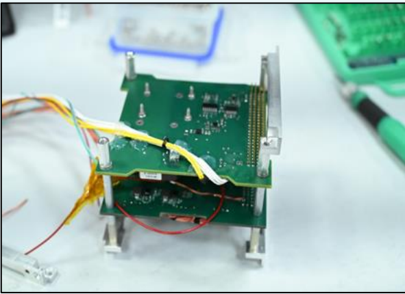
A student payload PCB stack taking shape in the SPACE lab
